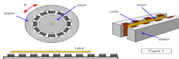
Figure 1-Linear Induction Motor
