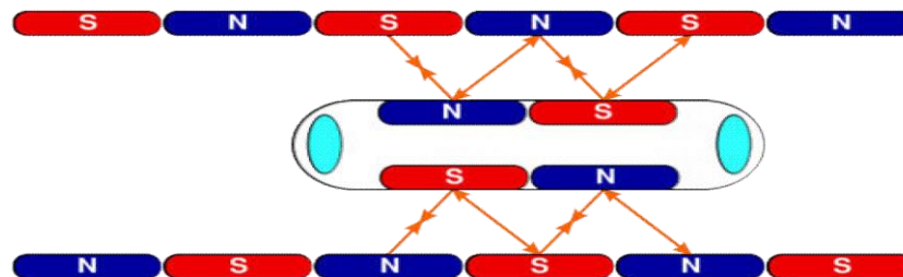
Figure 2- Magnetic Fields that moves the train forward
