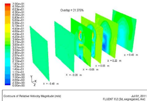
Figure 6 (c). Relative speed magnitude contour of the combined Darrieus-Savonius rotor for 21.37% overlap in YZ iso-planes
