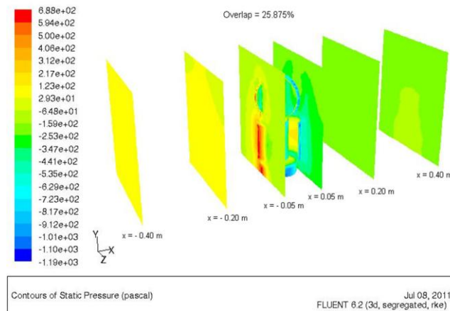
Figure 8 (d). Static pressure contour of the combined Darrieus-Savonius rotor for 25.87% overlap in YZ iso-planes
