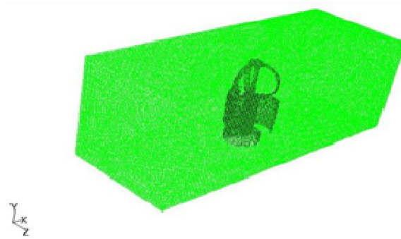
Figure 2 (b). Computational mesh of the combined Darrieus-Savonius rotor
