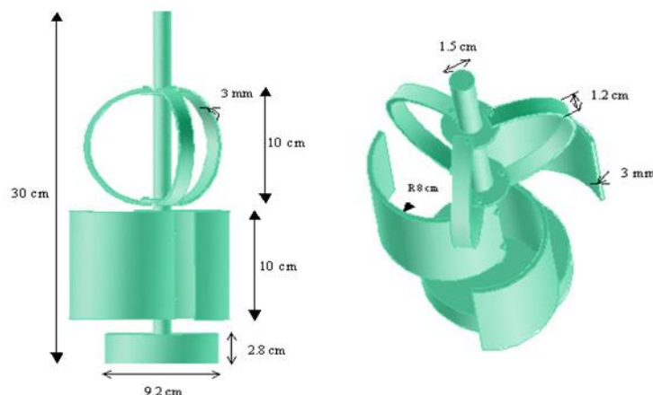
Figure1. Physical model of combined three-bladed-Darrieus-three-bucket Savonius rotor
