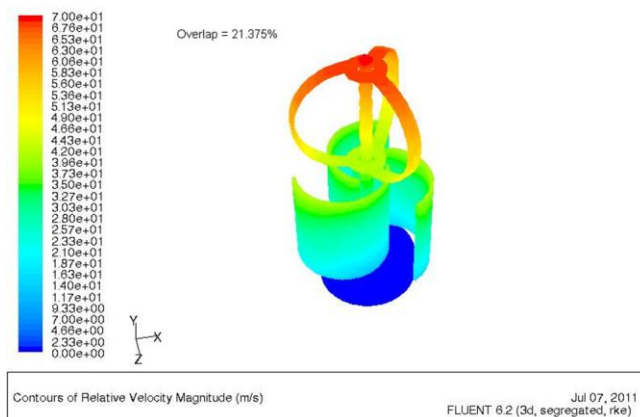
Figure 4 (c). Relative speed magnitude contour of the combined Darrieus-Savonius rotor for 21.37% overlap
