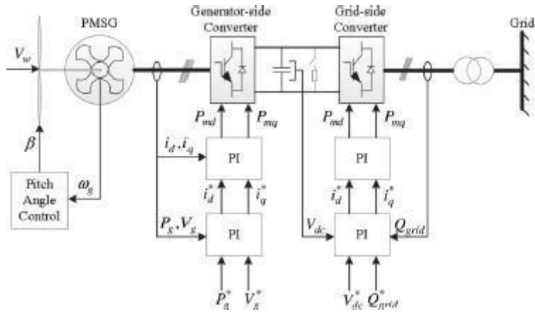
Fig 4: Modelling of DFIG based MCF
