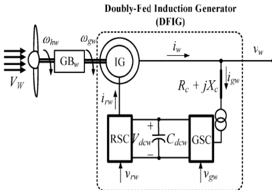
Fig 3: Schematic Diagram for DFIG
