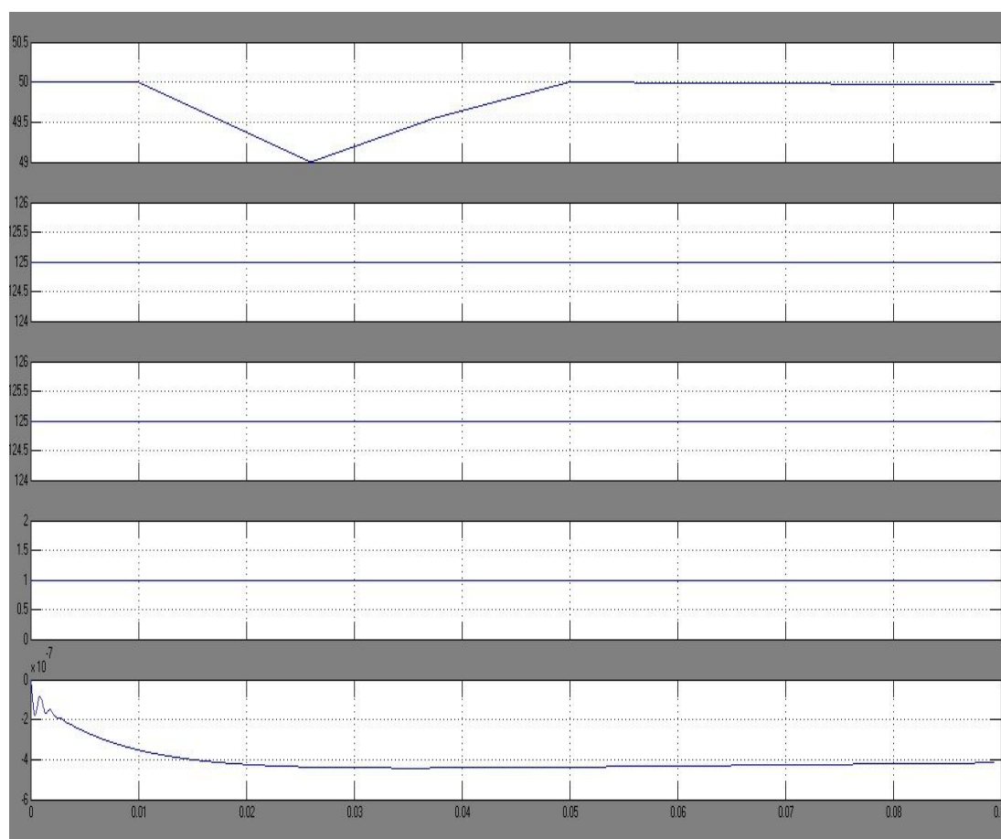
Figure 7: Simulation Result for (a) System Frequency, (b) Active Power, (c) Dc-link Voltage, (d) VSC active Power under normal frequency.
