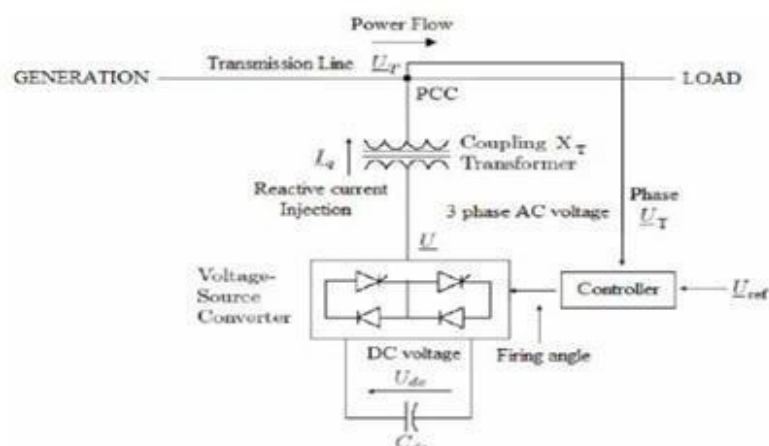
Fig 6: VSC-HVDC Controller
