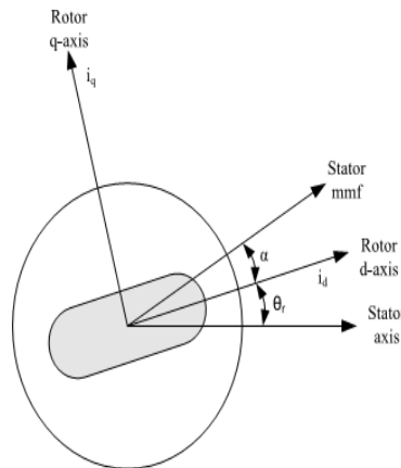
Fig 5: d-q model for the rotor reference frame
