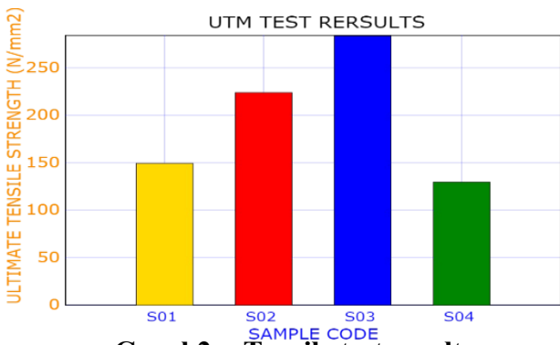
Graph2 : Tensile test results
