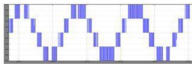
Fig. 21 Five level LSCPWM output
