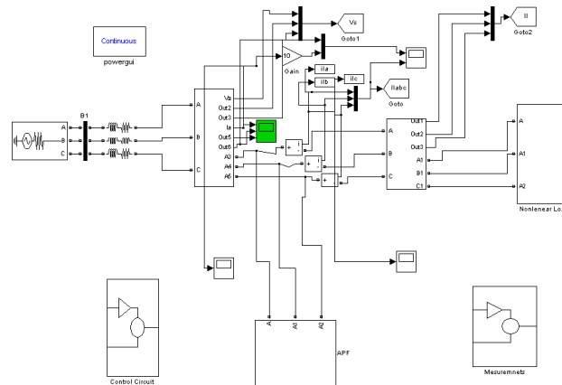
Fig. 9 Mat lab/Simulink power circuit model of D-STACTOM
