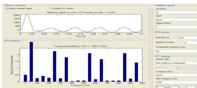
Fig. 20 Harmonic spectrum of Phase-A Source current without D-STACTOM
