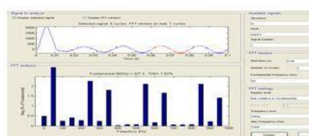
Fig. 27 Harmonic spectrum of Phase-A Source current with D-STATCOM
