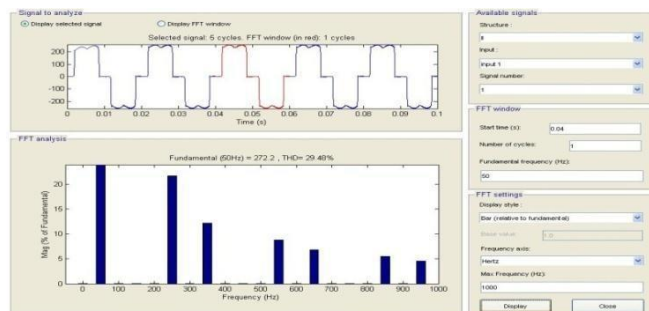
Fig. 15 Harmonic spectrum of Phase-A Source current without D-STACTOM
