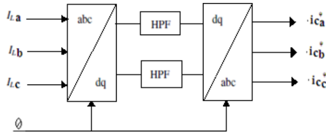
Fig. 3 Block Diagram of SRF method
