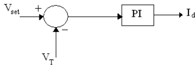
Fig. 2 PI Control Scheme
