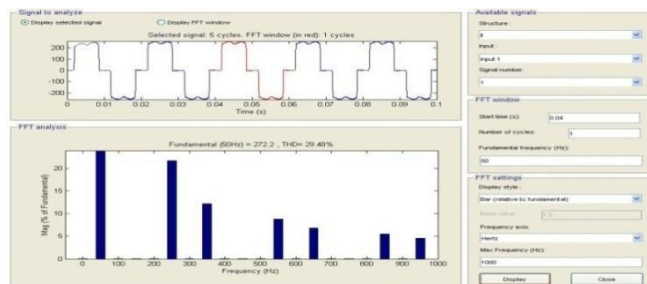
Fig. 19 Harmonic spectrum of Phase-A Source current without D-STACTOM
