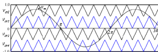
Fig.8 Level shifted carrier pulse width modulation.
