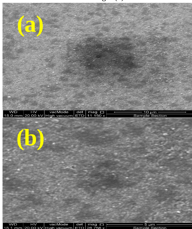
Fig. 2. Surface Morphology (Top-View) FESEM Image of Synthesized ZnO Thin Film (a) low Magnification and (b) High Magnification
