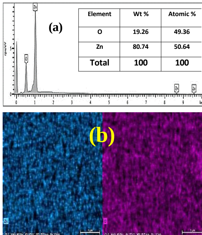
Fig. 3. (a) The EDX Spectrum Analysis of the synthesized ZnO Thin Film. (b) Elemental Mapping analysis for 3.7 Zinc:1Oxygen wt.% ratio for ZnO Thin Film Synthesized by using PVD Technique.
