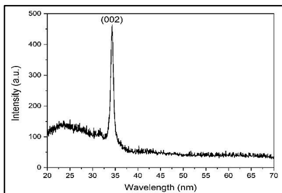
Fig. 4. XRD Pattern of Synthesized ZnO Thin Film
