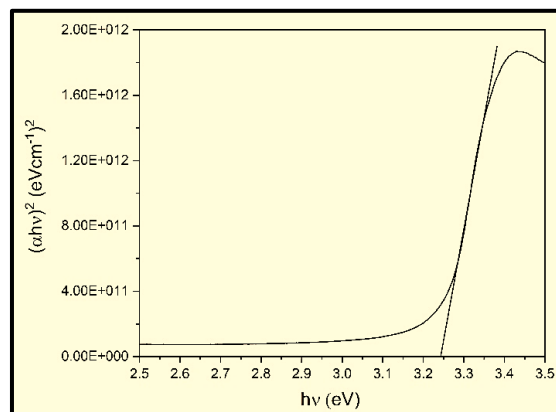
Fig. 6. Tauc plot (\alpha h\nu)^2 Versus Energy Band Gap (h\nu) of the ZnO Thin Film
