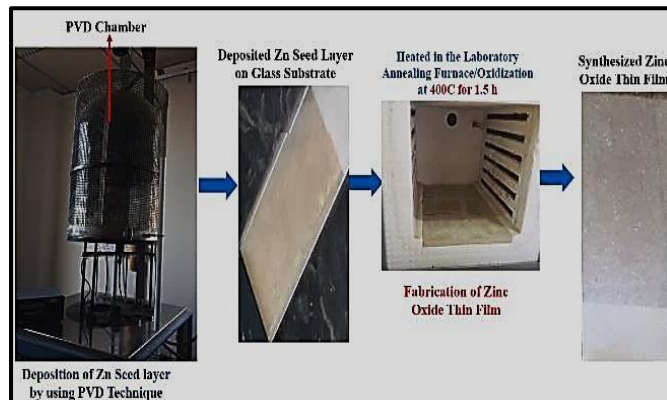
Fig. 1. Schematic Diagram of Synthesized ZnO Thin Film
