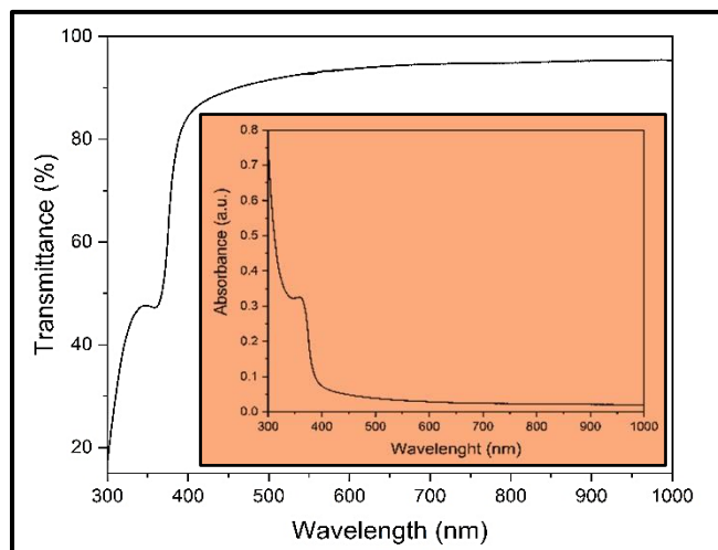
Fig. 5. Optical Transmission Spectrum of the Synthesized ZnO Thin film, the inset is Optical Absorption Spectrum of ZnO Thin Film.
