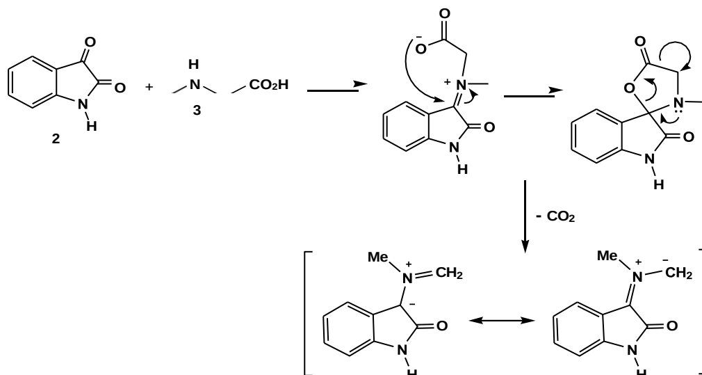
Figure 2. Mechanism for the generation of azomethine ylide
