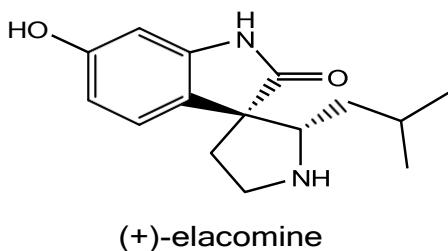
Figure 1. Representative naturally occurring spiropyrrolidinyl-oxoindole alkaloids
