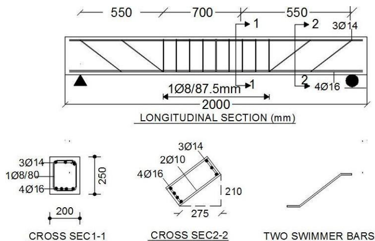
Fig. 4: Typical steel reinforcement used in this study
