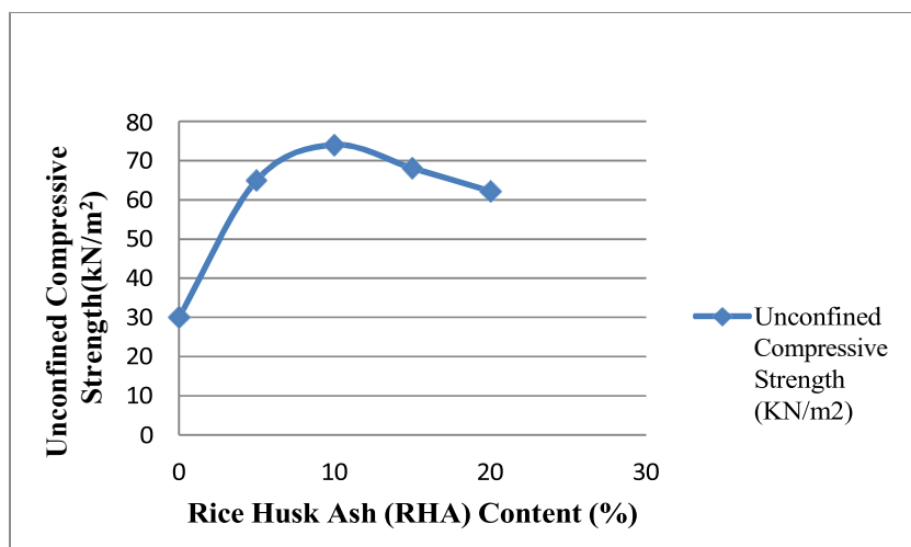
Figure 8 Comparative Effect of RHA on Unconfined Compressive Strength ( \text{kN/m}^2 ) of Black Cotton Soil
