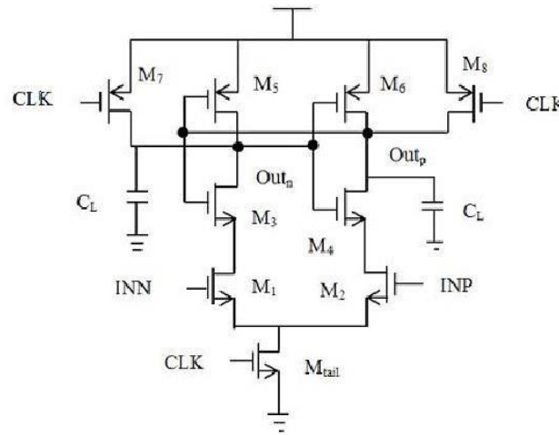
Figure 3: Fine Grain Single Tail Comparator
