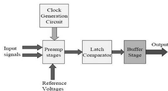
Figure 1: Comparator Architecture
