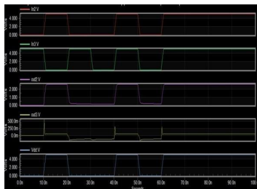
Simulation of Fine Grain Double Tail Comparator
