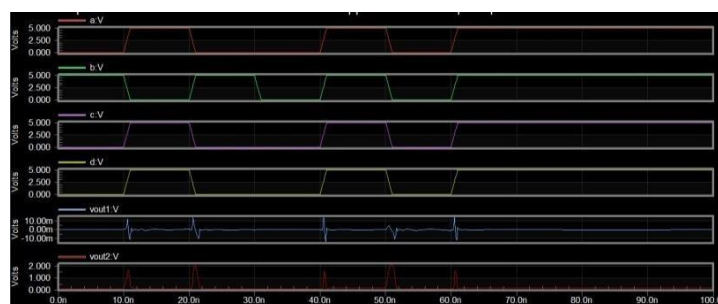
Simulation of Coarse Grain Double Tail Comparator
