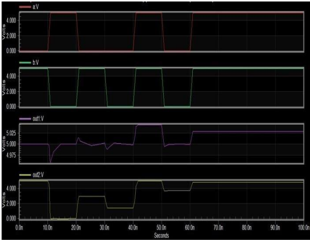
Simulation of Fine Grain single Tail Comparator
