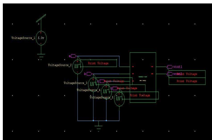
Extension Schematic of Coarse Grain Double Tail Comparator
