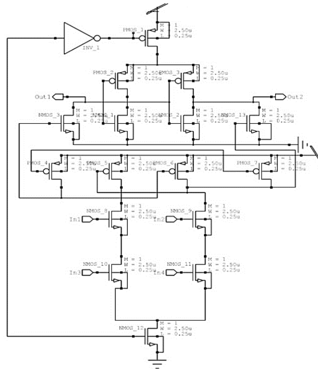
Figure 2: Coarse Grain Double Tail Comparator
