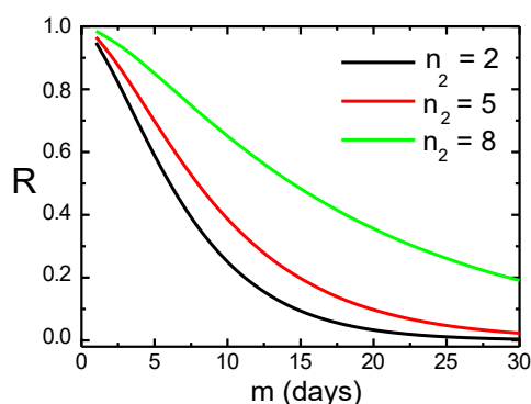
Figure 3: A plot of R versus m where R is the ratio of the number of symptomatic patients under lockdown to the number without lockdown (obtained from the present model), on the m^{\text{th}} day following the imposition of lockdown. Smaller values of n_2 indicate greater degree of social distancing.
