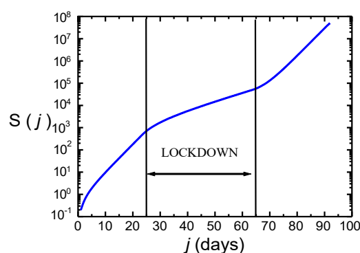
Figure 4: Variation of the number of symptomatic patients as a function of time for three phases: (i) before, (ii) during and (iii) beyond lockdown, assuming the lockdown to continue for 40 days (25 March to 03 May, 2020). Here, j = 1 on 01 March 2020 and j = 54 on 23 April 2020.
