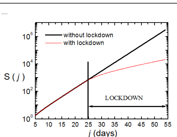
Figure 2: Variation of the number of symptomatic patients as a function of time, plotted in log scale. The red and black curves correspond to situations, with and without lockdown, respectively, as predicted by the present model. Here, j = 1 on 01 March 2020 and j = 54 on 23 April 2020.
