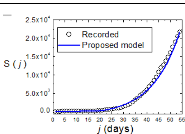
Figure 1: Variation of the number of symptomatic patients as a function of time. The circles denote the numbers registered in India during the period from 01 March 2020 (i.e. j = 1 ) to 23 April 2020 (i.e. j = 54 ). The continuous curve represents the values predicted by the present model.
