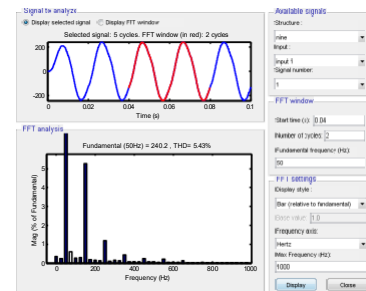
THD Analysis of output Voltage
