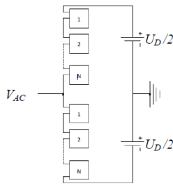
Figure 3.6 - Schematic of one phase of Multi-Level Converter.
