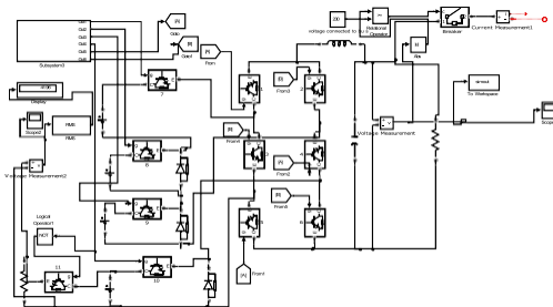
Simulation Circuit of Nine Level MMC
