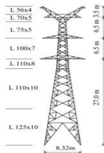
Fig no.2: Dimensions of Tower
