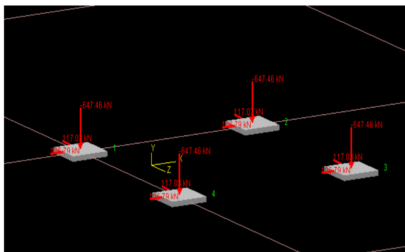
Fig no.9: Modeling of Isolated Footing in STAAD Foundation
