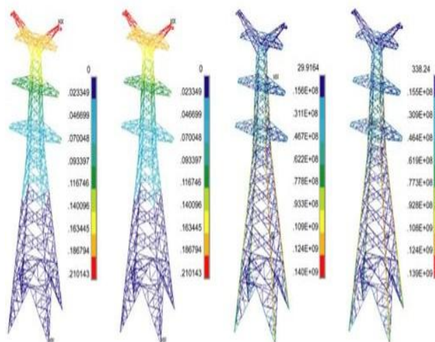
Fig no.3: Deflection and Stress plot
