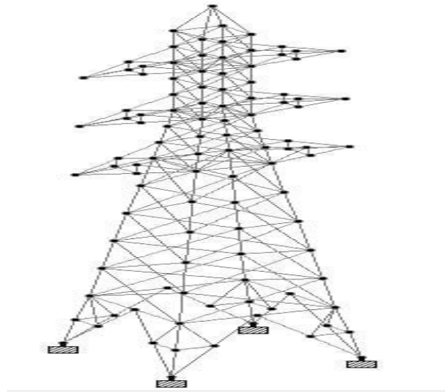
Fig no.6: Node Sketch in STAAD Pro
