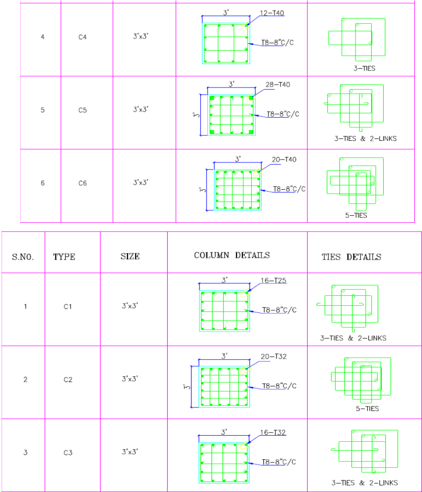
Fig:4.0:Area of steel reinforcement details in column
