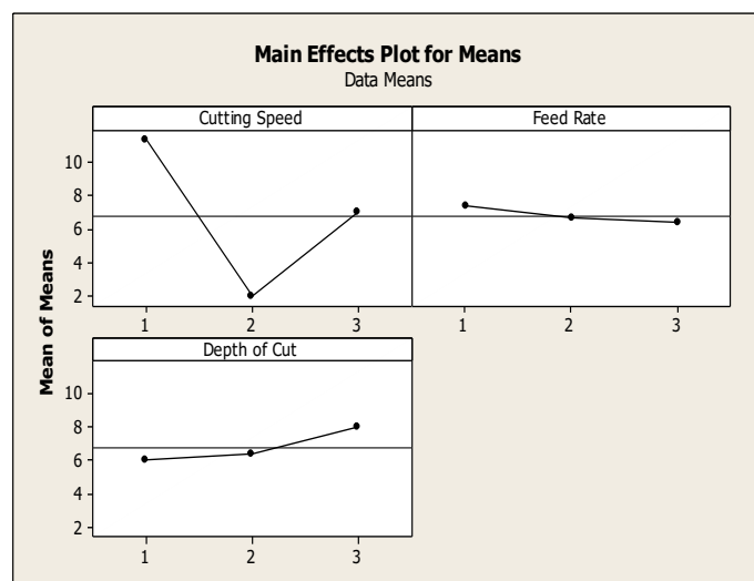
Fig 6.1 Tool Wear VS Cutting Speed, Depth of Cut and FeedRate
